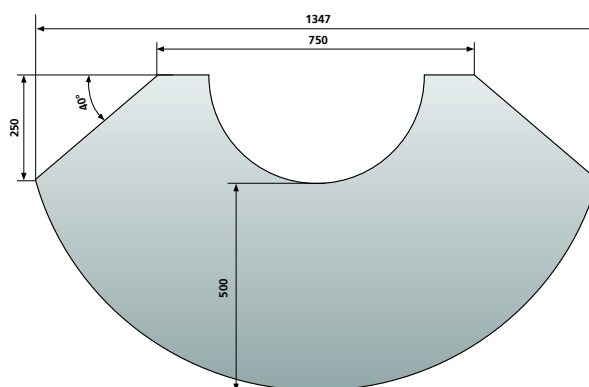
Plaque de sol avant, grand 1347 x 500 mm
